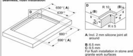
Measurements in mm Combination with electric hob Seamless, flush installation
