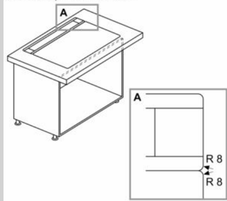
Combination with electric hob Seamless, flush installation
