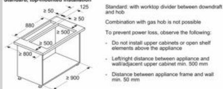
Measurements in mm Combination with electric hob Standard, top-mounted installation
