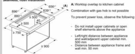
Measurements in mm Combination with electric hob Seamless, flush installation
