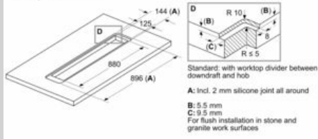
Measurements in mm Standard, flush installation
